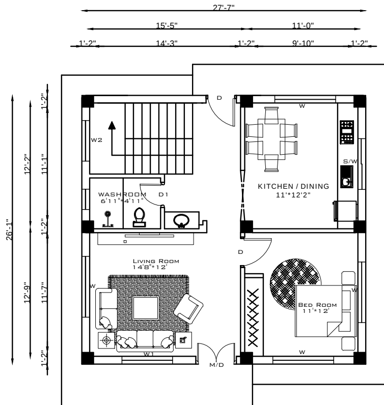
GROUND FLOOR PLAN AREA: 66.86 SQ.M.(719.41 SQ.F.)
