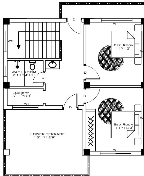
FIRST FLOOR PLAN AREA: 54.65 SQ.M.(588.03 SQ.F.)
